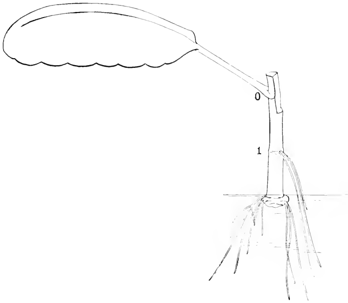
FIG. 89.—Stem with an apical leaf in which shoot formation is suppressed forms large amount of callus. Oct. 16 to Nov. 14, 1923.
